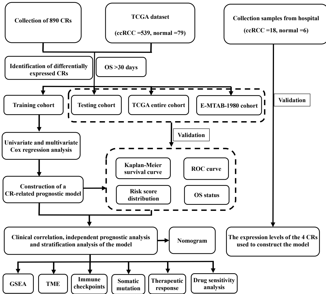
Figure S1 Study flowchart: overall study diagram. CRs, chromatin regulators; TCGA, The Cancer Genome Atlas; ccRCC, clear cell renal cell carcinoma; OS, overall survival; ROC, receiver operating characteristic; GSEA, Gene Set Enrichment Analysis; TME, tumor microenvironment.
