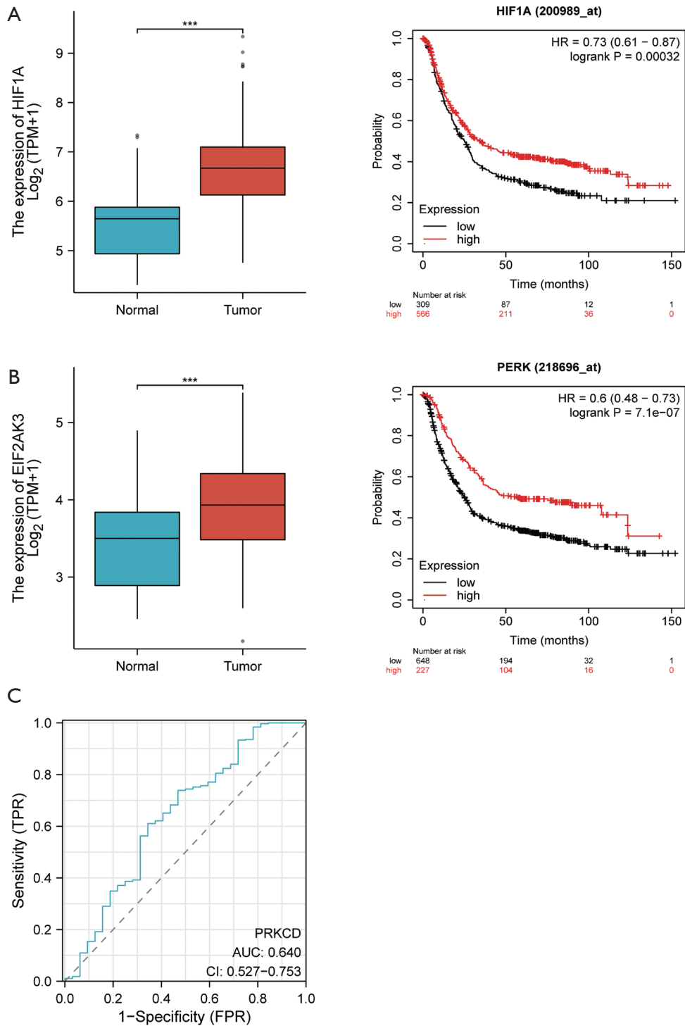
Figure S1 Overall survival curves and receiver operating characteristic (ROC) curves for HIF1A , EIF2AK3 , and PRKCD in gastric cancer. (A) Expression of HIF1A in gastric cancer; lower expression of HIF1A leads to shorter overall survival. (B) Expression of EIF2AK3 ( PERK ) in gastric cancer; lower expression of EIF2AK3 ( PERK ) leads to shorter overall survival. (C) The ROC curve analysis demonstrated that PRKCD possesses an area under the curve (AUC) of 0.640.
