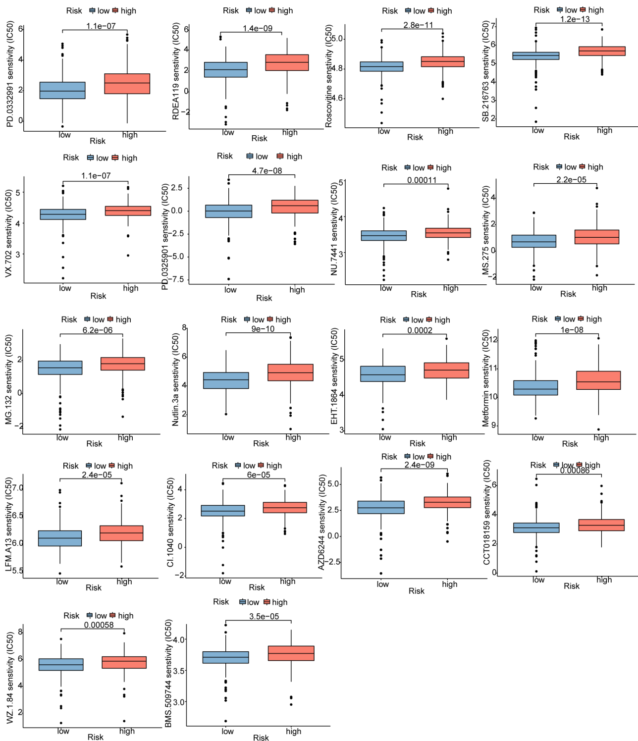
Figure S6 Compounds with lower IC50 in low-risk group. IC50, lower half maximal inhibitory concentration.
