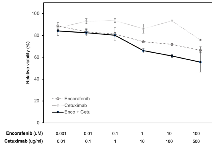
Figure S1 Encorafenib and cetuximab dual combination has no synergistic impact on PDC viability. BRAF V600E-mutant CRC PDCs were treated with indicated drugs for 24 h. Then, the number of viable cells was determined using a CellTiter 96 AQueous One Solution Cell Proliferation Assay (MTS) and viability was calculated as a percent of the untreated control. No statistical differences were uncovered between the experimental groups when tested using ANOVA with Tukey-adjusted post hoc tests for multiple comparisons. PDC, patient-derived cell; CRC, colorectal cancer; ANOVA, analysis of variance.
