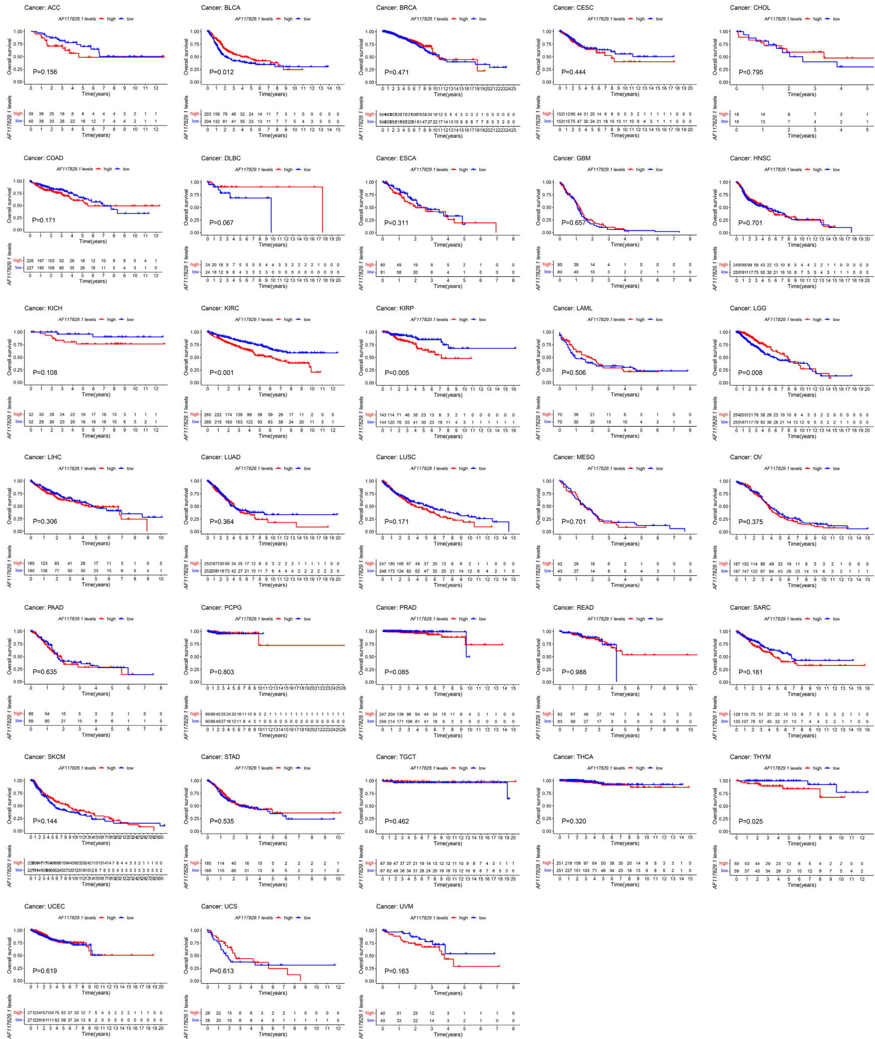
Figure S1 Prognostic value of AF117829.1 on overall survival for pan-cancer with Kaplan-Meier plotter.
