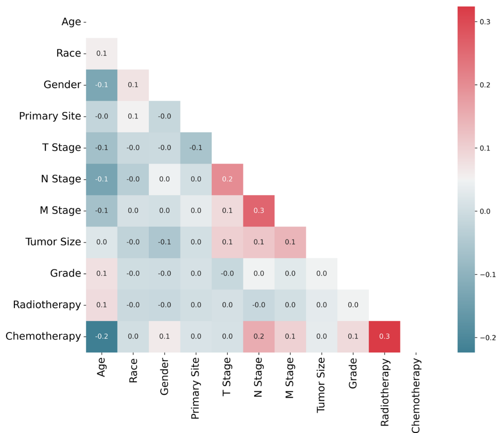
Figure S2 The results of Spearman correlation analysis between all the independent variables. The heatmap shows the correlation between the variables.
