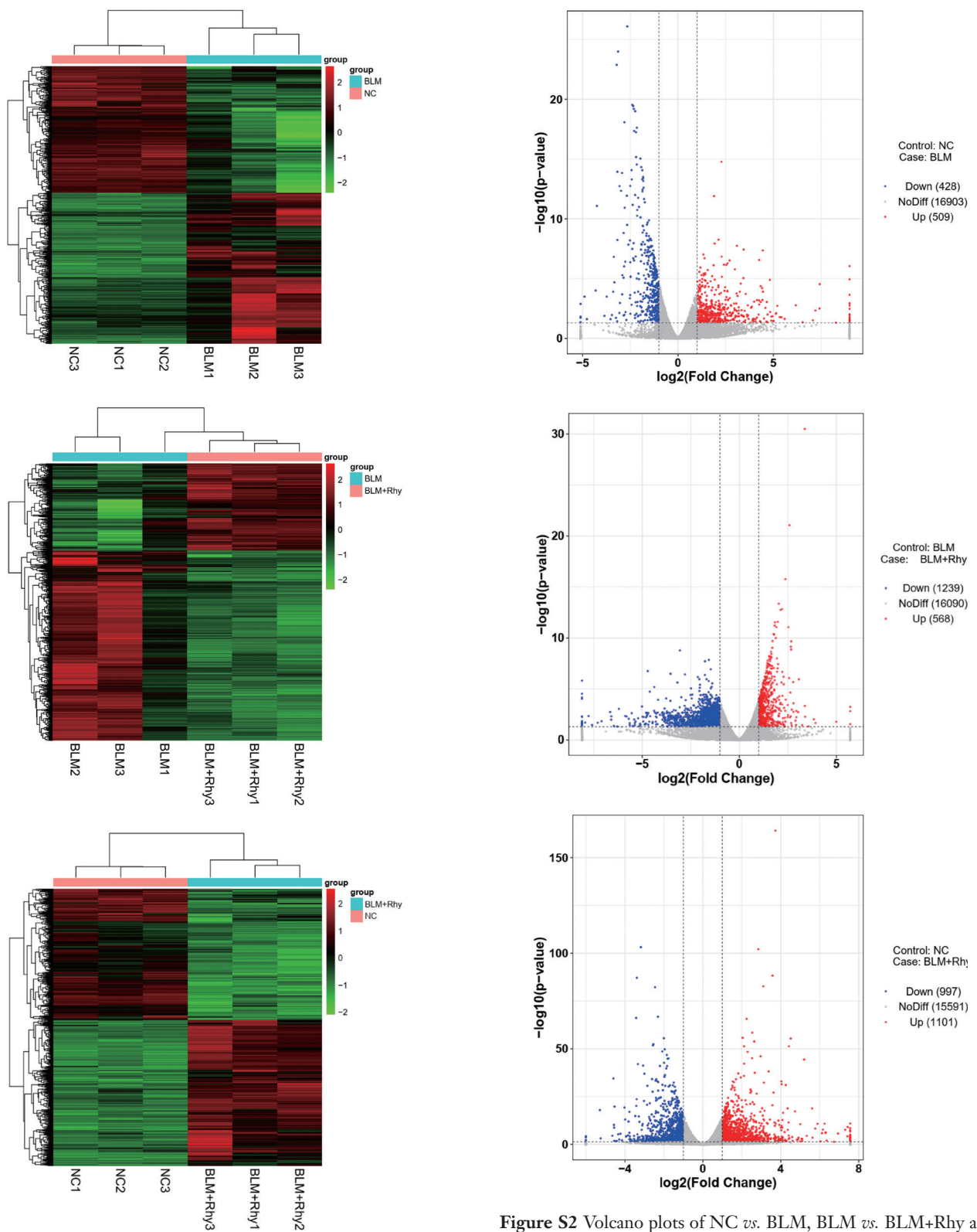
Figure S1 The heatmaps of differentially expressed genes in NC vs. BLM, BLM vs. BLM+Rhy and NC vs. BLM+Rhy groups.
