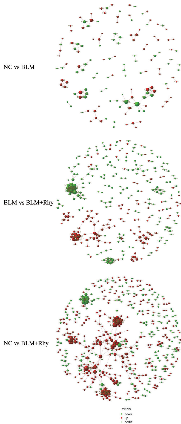
Figure S5 PPI of differentially expressed mRNAs of NC vs. BLM, BLM vs. BLM+Rhy, NC vs. BLM+Rhy groups.
