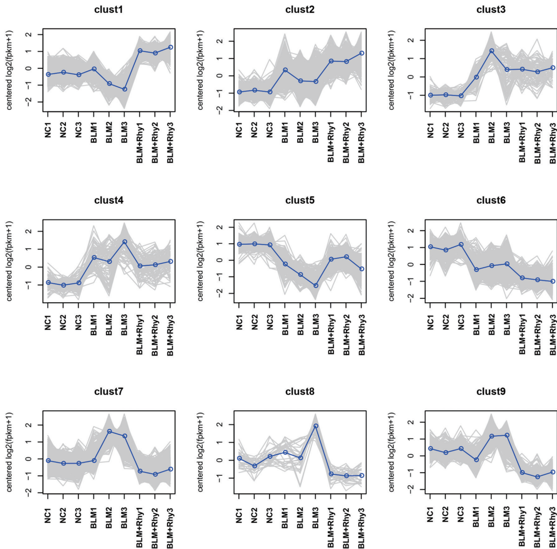
Figure S6 Expression patterns of genes of NC, BLM and BLM+Rhy groups in nine clusters.
