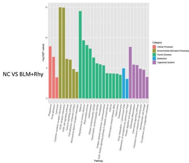
Figure S3 KEGG analysis of NC vs. BLM, BLM vs. BLM+Rhy and NC vs. BLM+Rhy groups.
