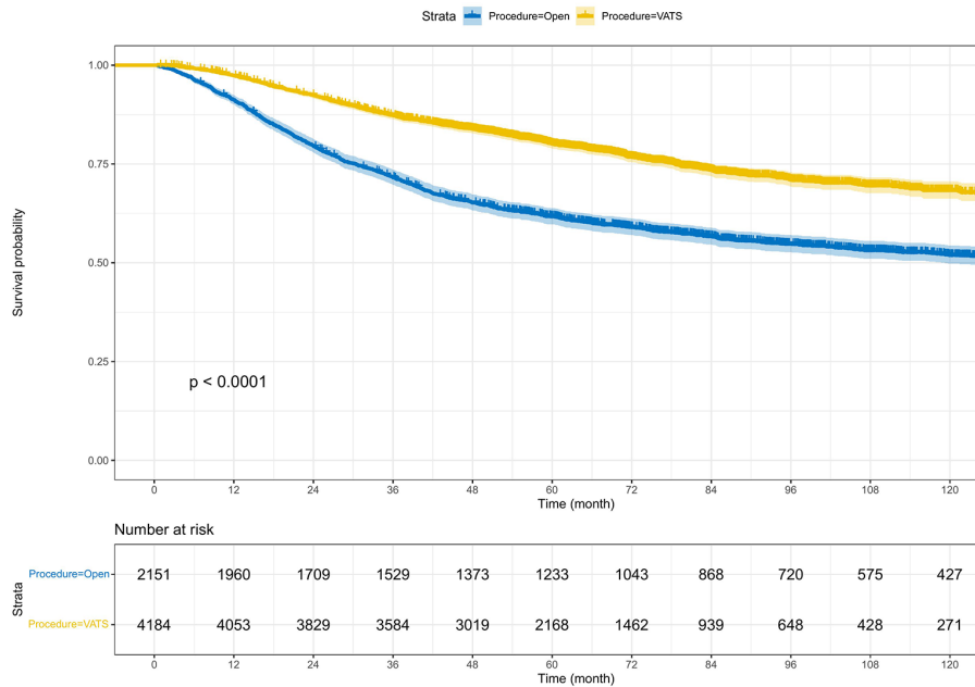
Figure S1 Lung cancer-specific survival of p-stage I–III NSCLC patients stratified by VATS vs. open lobectomy. NSCLC, non-small cell lung cancer; VATS, video-assisted thoracic surgery.
