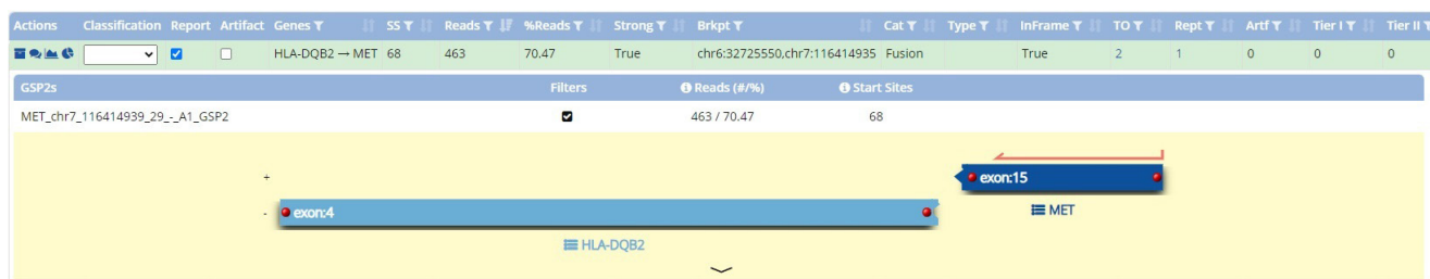
Figure S1 The breakpoints in the genomic DNA sequence that show the HLA-DQB2::MET fusion points.
