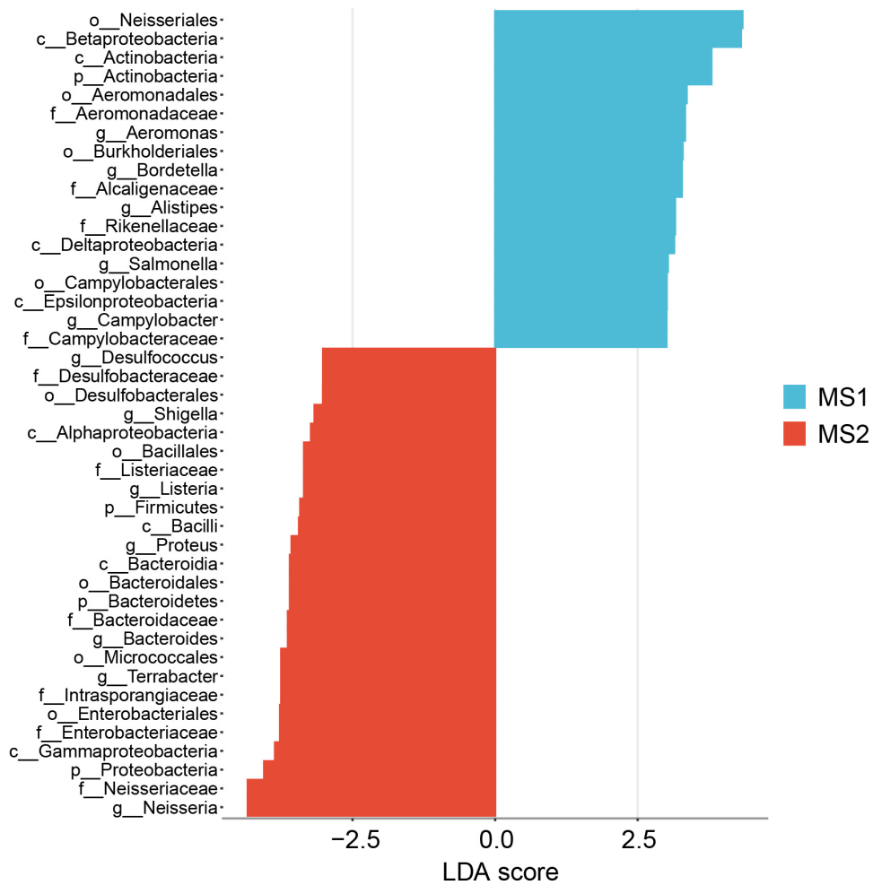
Figure S2 Histogram of the linear discriminant analysis combined with effect size. The LDA score indicates the effective size and ranking of each differential abundant taxon ( |LDA\ score| > 3 ). The “p” indicate phylum, the “c” indicate class, the “o” indicate order, the “f” indicate family, and the “g” indicate genus.
