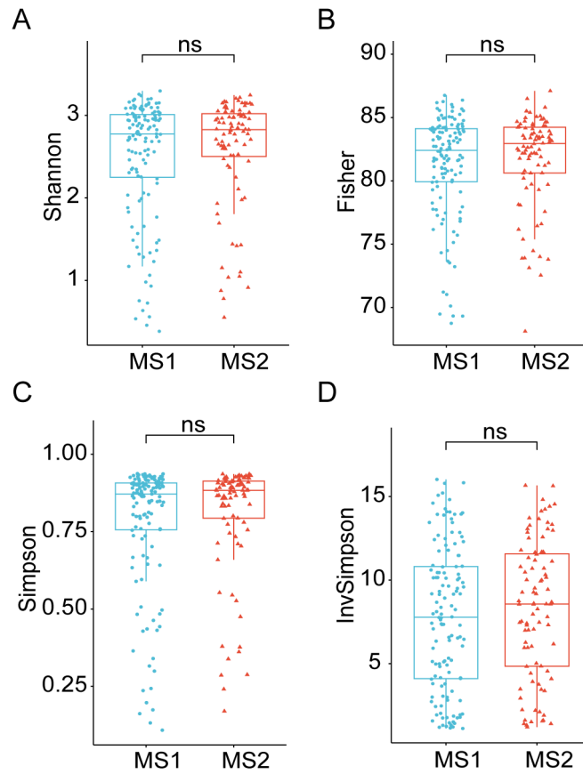
Figure S1 The \alpha -diversity index in MS1 and MS2. (A) Shannon index in MS1 and MS2 groups. Asterisks are labeled according to the P values calculated, the same below. (B) Fisher index in MS1 and MS2 groups. (C) Simpson index in MS1 and MS2 groups. (D) InvSimpson index in MS1 and MS2 groups. MS1, molecular subtype 1; MS2, molecular subtype 2.
