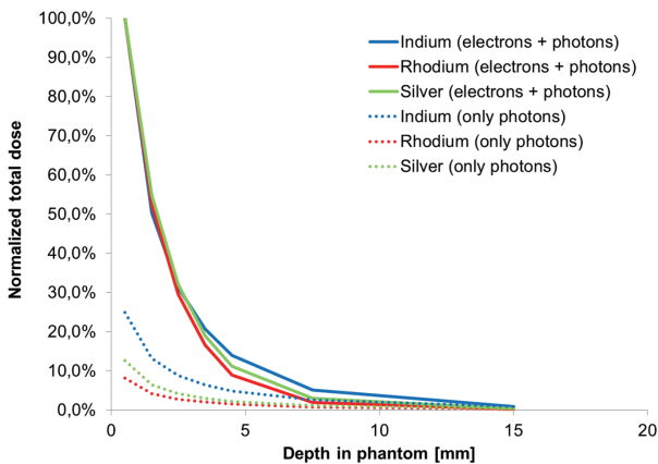
Figure S2 Continued lines: BE in-depth total dose rates profiles comparison in a polystyrene phantom at the RA-6 BNCT beam (normalized to the first millimeter total dose of each BE). Dotted lines: photon dose component of each BE.
