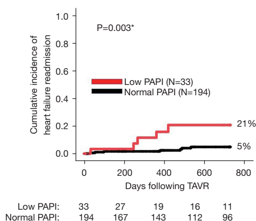
Figure 2 Cumulative incidence of the primary endpoint stratified by the level of baseline PAPI. *, P < 0.05 by log-rank test. TAVR, transcatheter aortic valve replacement; PAPI, pulmonary artery pulsatility index.
